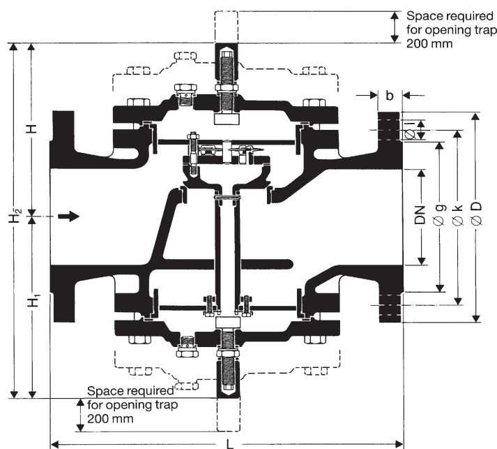
TK 23 and TK 24, DN 65-100 mm (2½-4")
