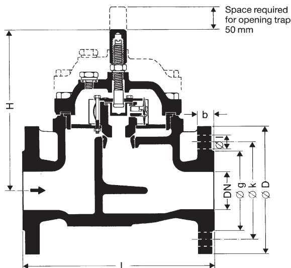
TK 23 and TK 24, DN 50 mm (2")
