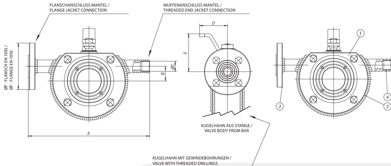
Abmessungen / Dimensions [mm]
